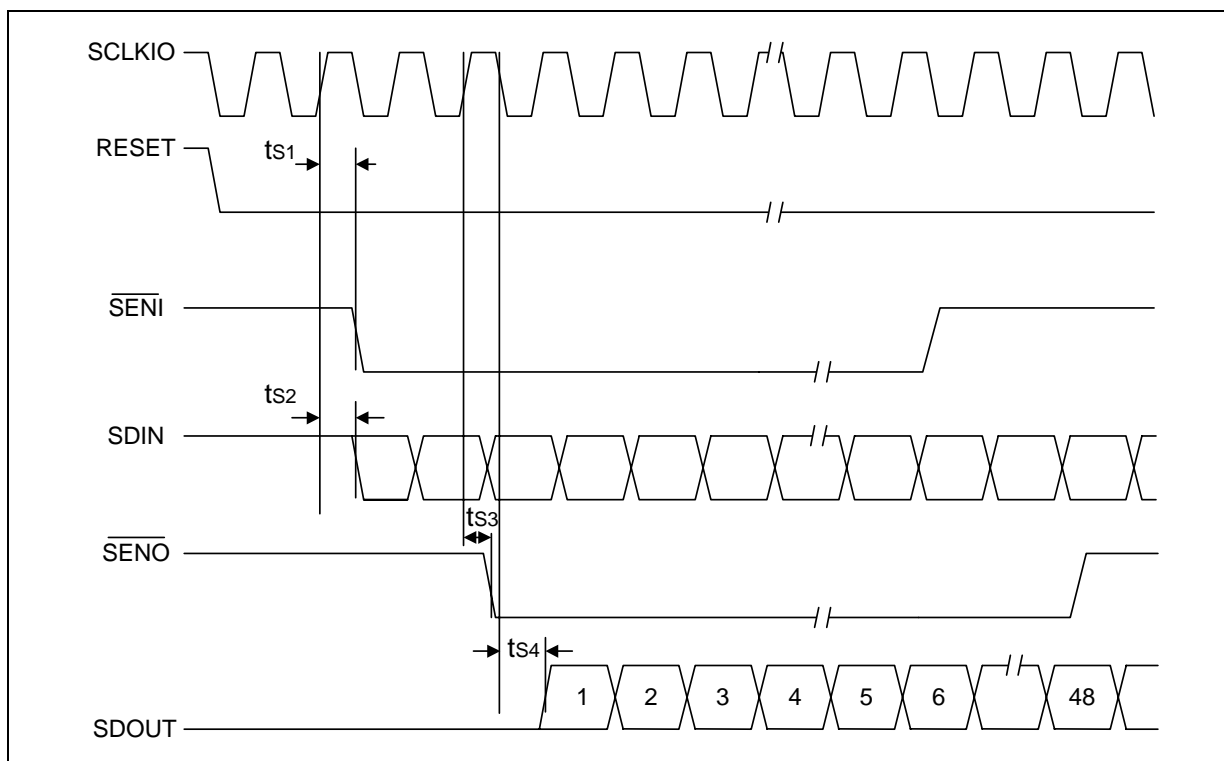
Figure 12. Serial Port Timing
