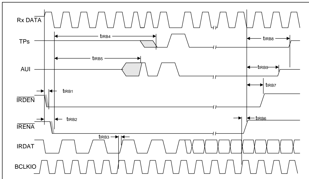
Figure 13. Inter-Repeater Bus Timing
